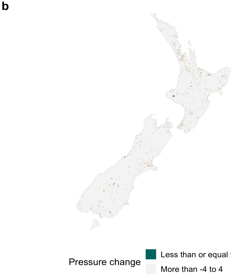
Appendix S1: difference between the local layers (2012 and 2018); (a) shows a histogram of difference in pressures between 2012 and 2018. The dashed vertical lines are at -4, 4; in (b) pressure values outside of -4, 4 are shown in the map as green and brown respectively. We refer to the main text for the average difference.
